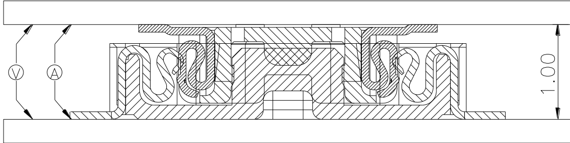
Figure 1 (P/N: 5.005/5.016)
